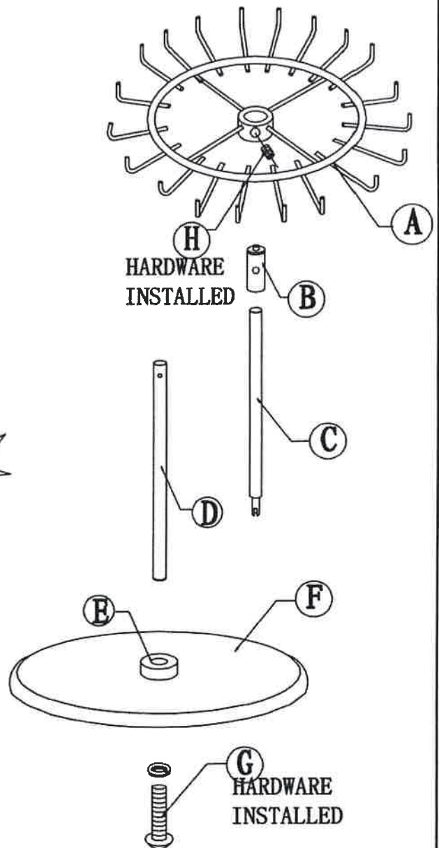
ASSEMBLY EXPLODED VIEW
