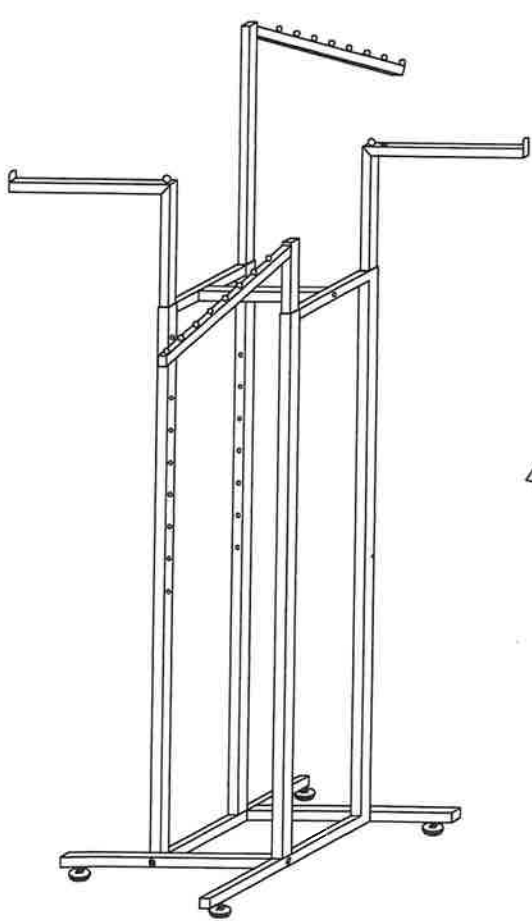
ASSEMBLING DRAWING
