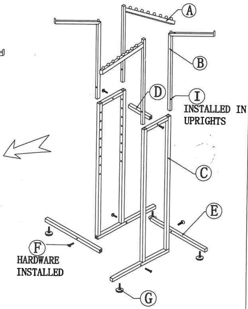
ASSEMBLY EXPLODED VIEW
