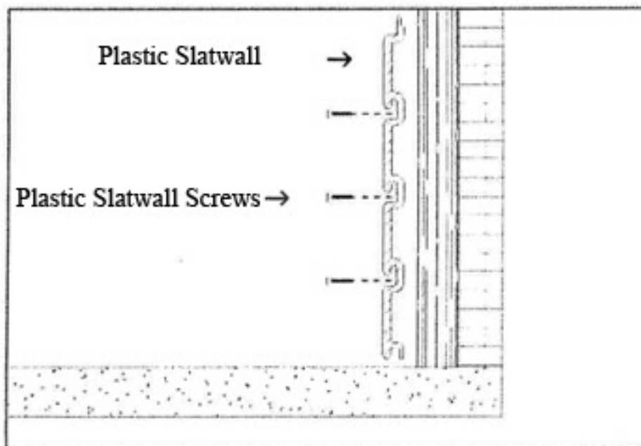
Figure 2. Plastic slatwall installation.
